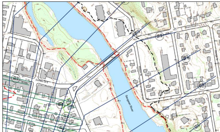
FLOODPLAIN LIMITS AT BRIDGE
