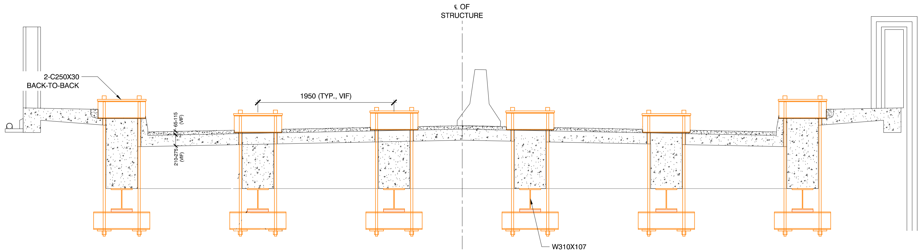
2 GIRDER SHORING DETAIL S2 SECTION
